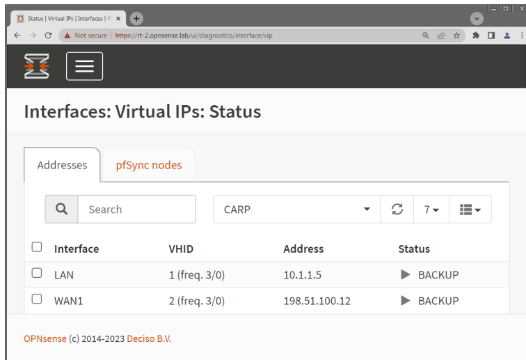
Figure 12.3: Firewall RT-2 becomes CARP Backup
