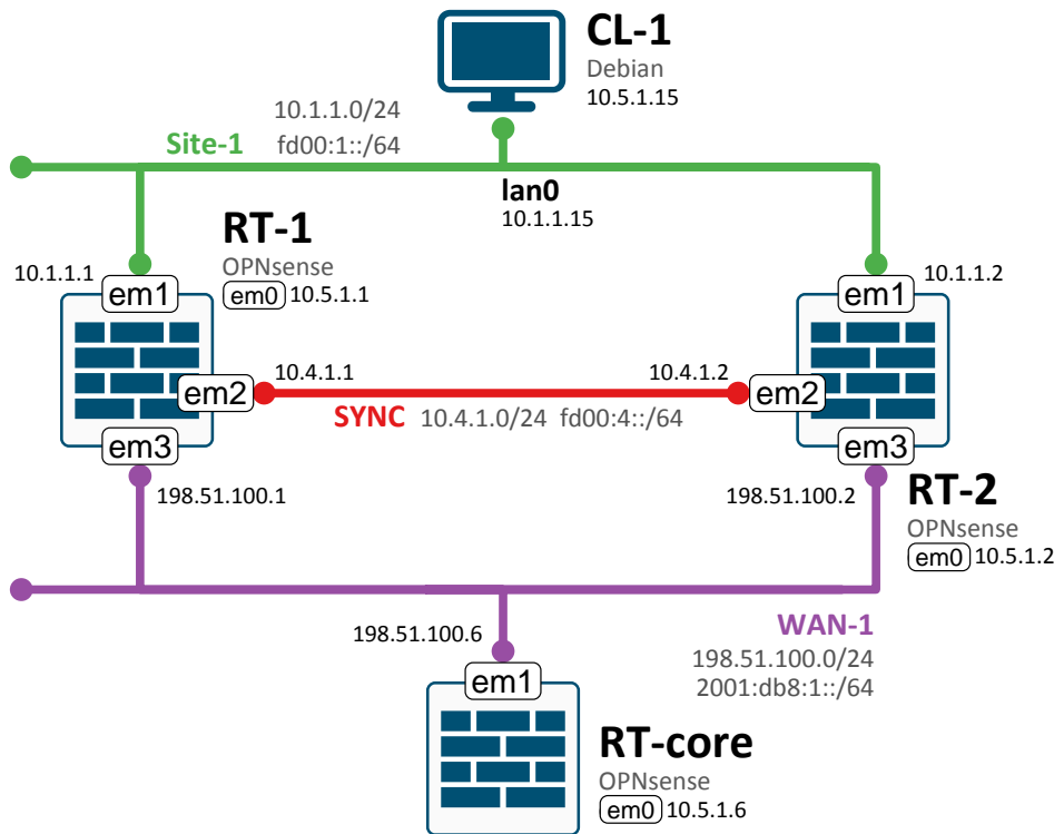
Figure 12.1: The firewalls RT-1 and RT-2 build a CARP cluster
