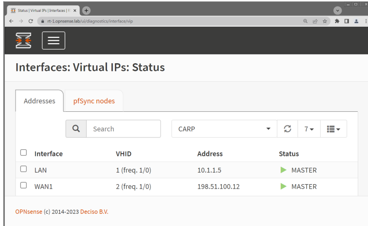
Figure 12.2: Firewall RT-1 becomes CARP Master
