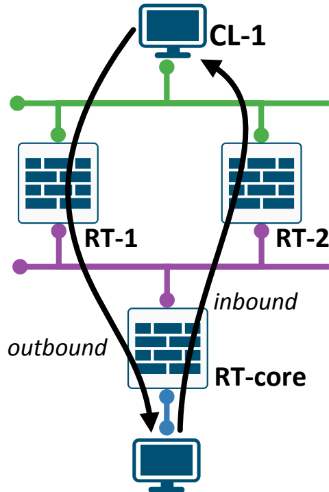
Figure 12.6: CARP might introduce asymmetric routing
