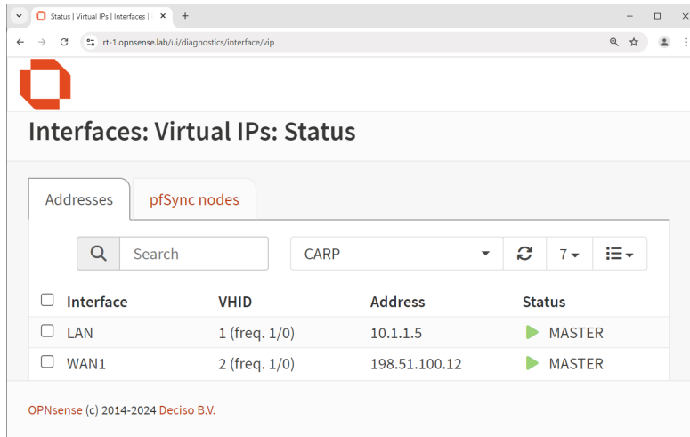
Figure 12.2: Firewall RT-1 becomes CARP Master
