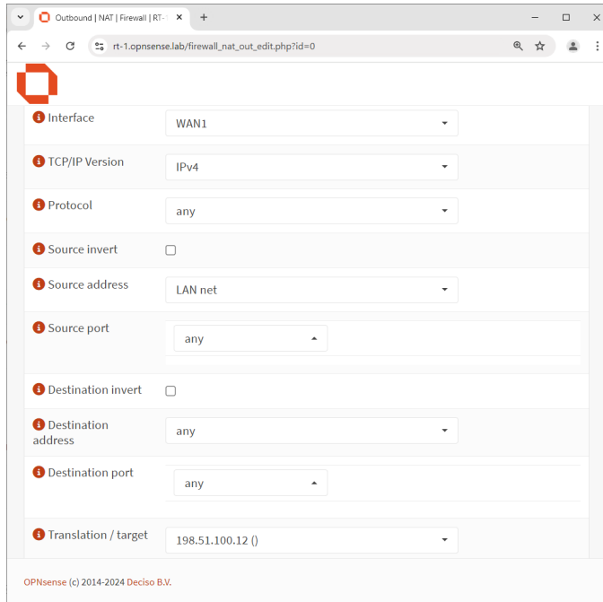
Figure 12.4: Firewall RT-1 translates IPv4 addresses
